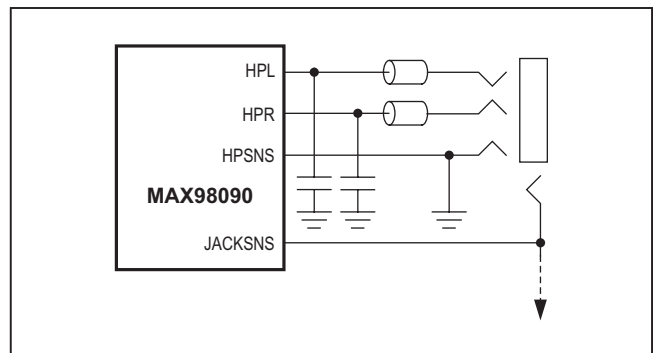
Figure 56. Optional Class H Output Filter
