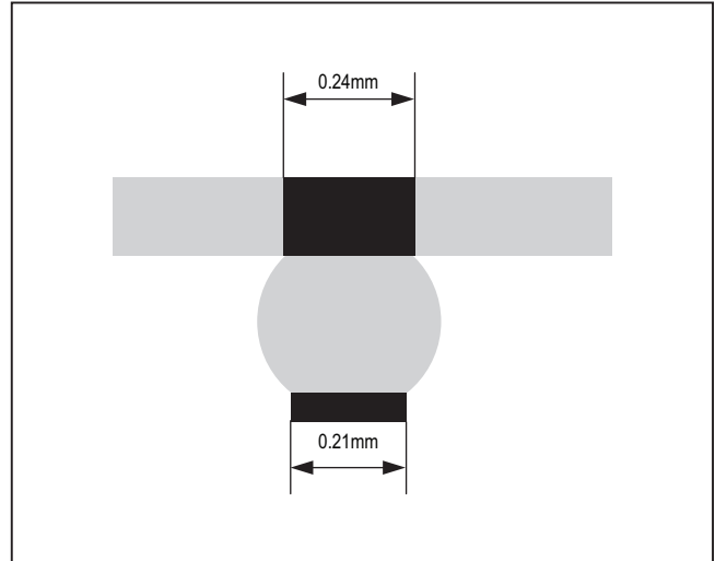
Figure 58. WLP Package Ball Dimensions
