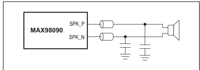
Figure 55. Optional Class D Ferrite Bead Filter
